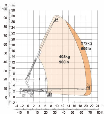
85-J Diesel DUAL REACH / 85-J Hybrid DUAL REACH Telescopic Boom mode
