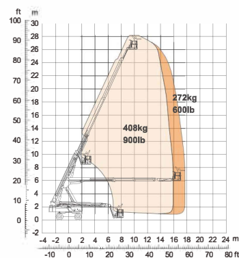
85-J Diesel DUAL REACH / 85-J Hybrid DUAL REACH Articulated Boom mode
